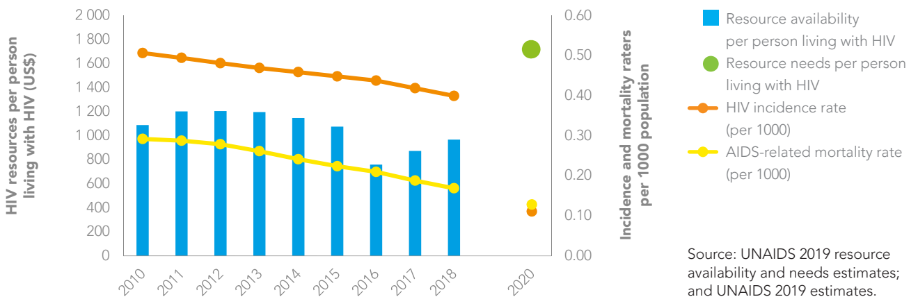
FIGURE 9.9 Total HIV resource availability per person living with HIV in constant 2016 US dollars, HIV incidence and AIDS-related mortality rates (per 1000), low- and middle-income countries in the Caribbean, 2010–2018 and 2020 targets
